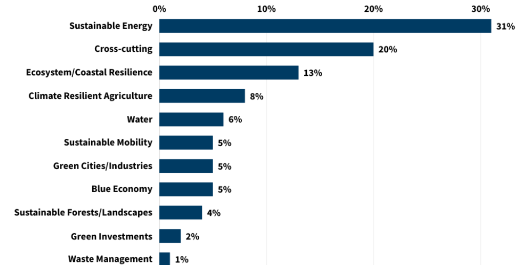
Pacific Pipeline, Project Breakdown By Thematic Impact Area
