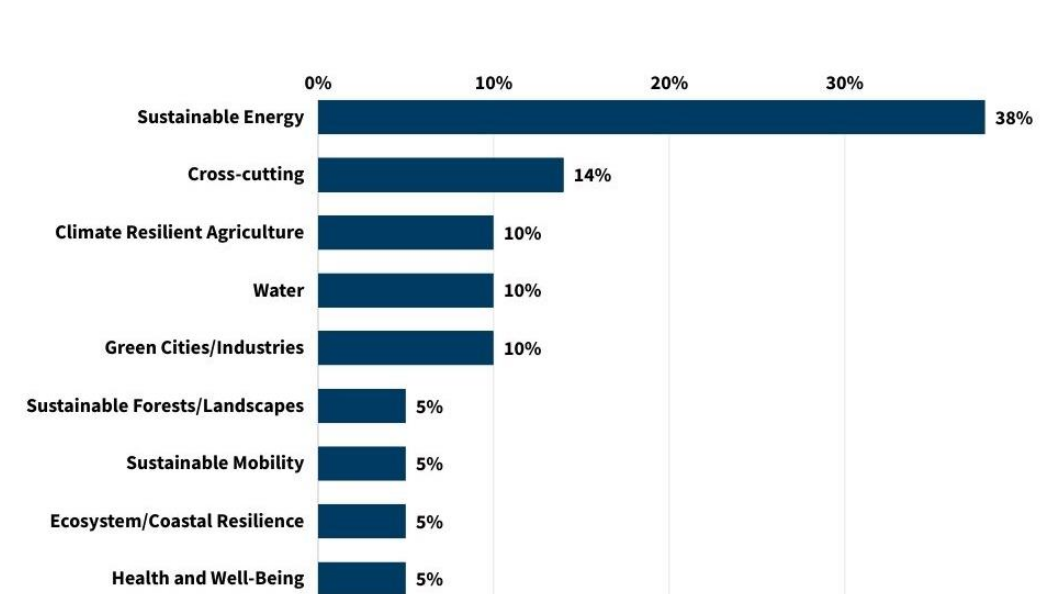
Caribbean Pipeline, Project Breakdown By Thematic Impact Area
