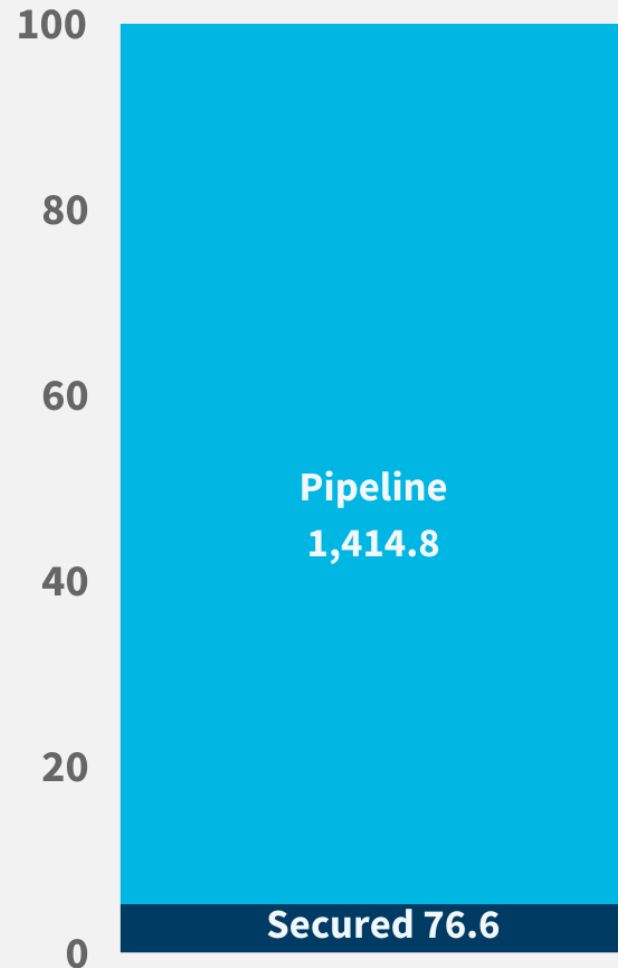
GLOBAL TOTAL BY STATUS
