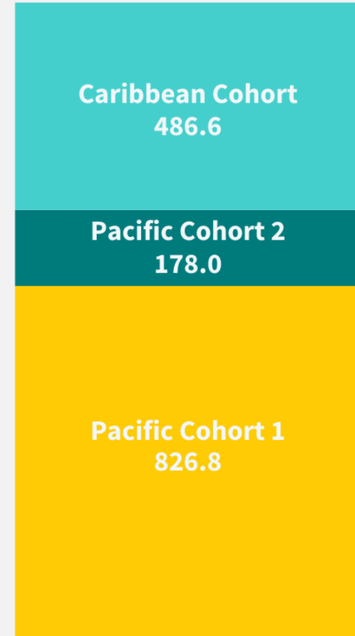
GLOBAL TOTAL BY REGION
